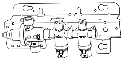
Hose/90 Stop Lead Free TMA (S45-2730)
